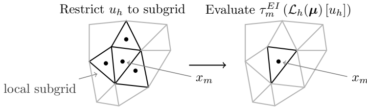
FIGURE 4.1. Illustration of finite volume operator evaluation on a local subgrid
