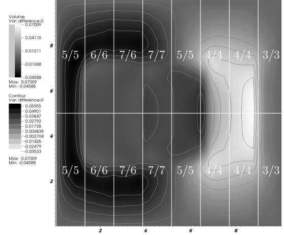
Figure 2: Difference between fine scale and reduced solution from Figure 1 and coarse triangulation (white) with number of reduced basis functions |\Phi_F| for each coarse cell F for the fine triangulation with 2048 and 32768 cells.
