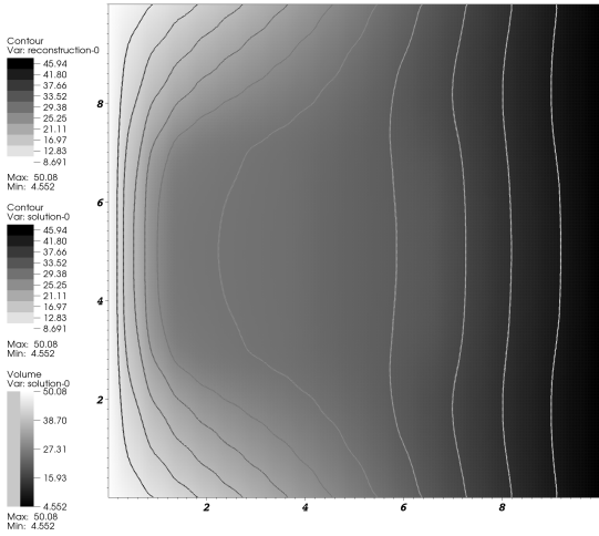
Figure 1: Contour plots of fine scale solution (solid lines) and reconstructed reduced solution (dotted lines) to Equation (1) for \mu_1 = 0.85 , \mu_2 = 0.5 , \mu_3 = 0.1 , volume representation of reconstructed reduced solution. Here: |\mathcal{T}_h| = 32768 .
