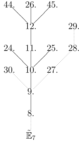
Figure 3: \geq \tilde{\mathbb{E}}_7
