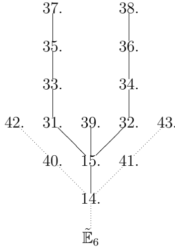
Figure 2: \geq \tilde{\mathbb{E}}_6
