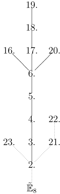
Figure 4: \geq \tilde{\mathbb{E}}_8
